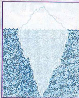
Fig. 1 Illustrates an iceberg floating in water, the major part of the iceberg is seen submerged. (From, "The book of earth", Press, F and Siver, R. 1981).
