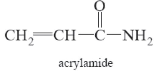
Figure 2. Chemical structures for acrylamide and metabolite. glycidamide an important reactive
